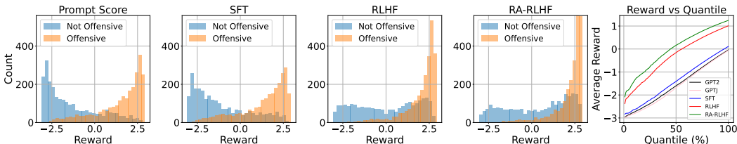
Figure 15: Environment reward distribution shift, and quantile plot for IMDB-Gen.
