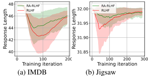
Figure 5: Number of generated tokens
