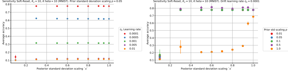
Figure 13: Soft Reset , K_\gamma = 10, K_\theta = 10 , sensitivity analysis of performance with respect to the hyperparameters on data-efficient random-label MNIST. The x-axis denotes the studied hyperparameter, whereas the y-axis denotes the average performance across the tasks. The standard deviation is computed over 3 random seeds. The color indicates additional studied hyperparameter. (Left) shows sensitivity analysis where the x-axis is the posterior standard deviation scaling s and the color indicates the drift model learning rate \eta_\gamma . (Right) shows sensitivity analysis where the x-axis is the posterior standard deviation scaling s and the color indicates initial prior standard deviation scaling \nu .
