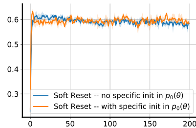
Figure 23: Impact of specific initialization \theta_0 as a mean of p_0(\theta) in Soft Resets . The x-axis represents task id. The y-axis represents the average task accuracy with standard deviation computed over 3 random seeds. The task is random label MNIST – data efficient.
