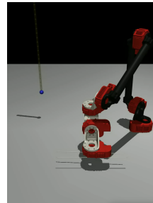
Figure 3: TychoEnv Reach Task Setup We aim to compare our approach of exploration policy transfer with direct sim2real policy transfer. To this end, we first train a policy in \mathcal{M}^{\text{sim}} that solves the task in \mathcal{M}^{\text{sim}} , \pi^{\text{sim},*} , and then utilize this policy in place of \Pi_{\text{exp}} in Algorithm 2. We instantiate our approach of exploration policy transfer as outlined above. Our aim in this experiment is to illustrate how the quality of the data provided by direct policy transfer vs. exploration policy transfer affects learning. As such, for both approaches we simply initialize our SAC agent in \mathcal{M}^{\text{real}} , \mathfrak{A}_{\text{po}} , from scratch, and set the reward in \mathcal{M}^{\text{real}} to be sparse: the agent only receives a non-zero reward if it successfully touches the ball. For each approach, we repeat the process of training in \mathcal{M}^{\text{sim}} four times, and for each of these run them for two trials in \mathcal{M}^{\text{real}} .
