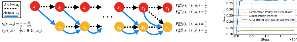
Figure 2: Left: Illustration of Combination Lock Example. Right: Results on Combination Lock.
