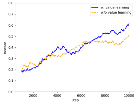
Figure 7: Learning curves with and without value learning, trained on the Drawbench prompt set: Adding value learning could result in higher reward using less time.
