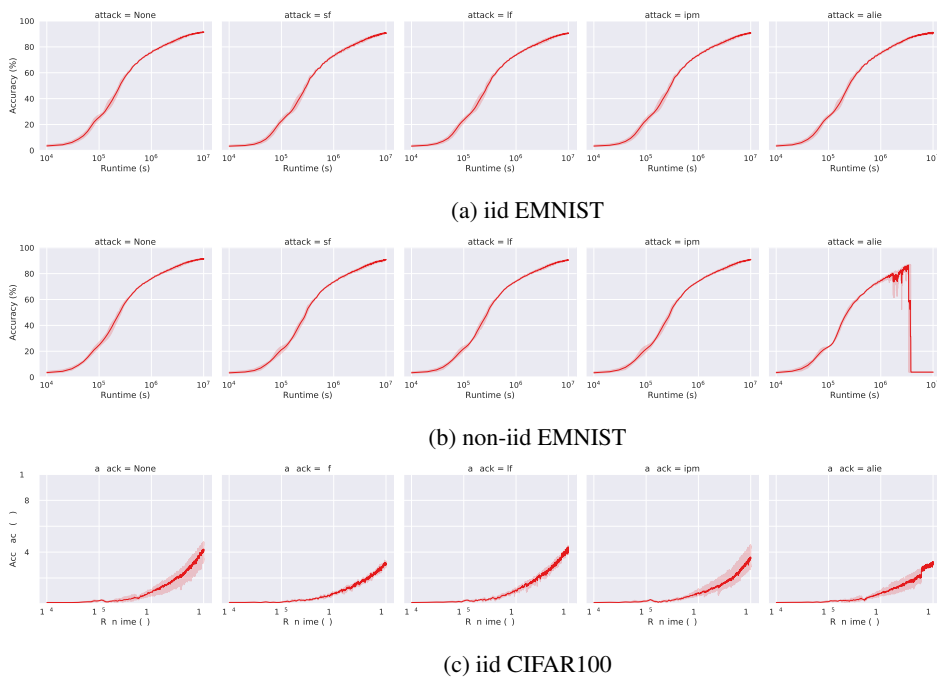
Figure 13: The accuracy achieved by CC in a given setting. A cohort size of 50 peers was used, with 10 malicious workers. Each algorithm was run for 1000 rounds, with 0.9 momentum, 1000.0 \epsilon , and for 3 different seeds.
