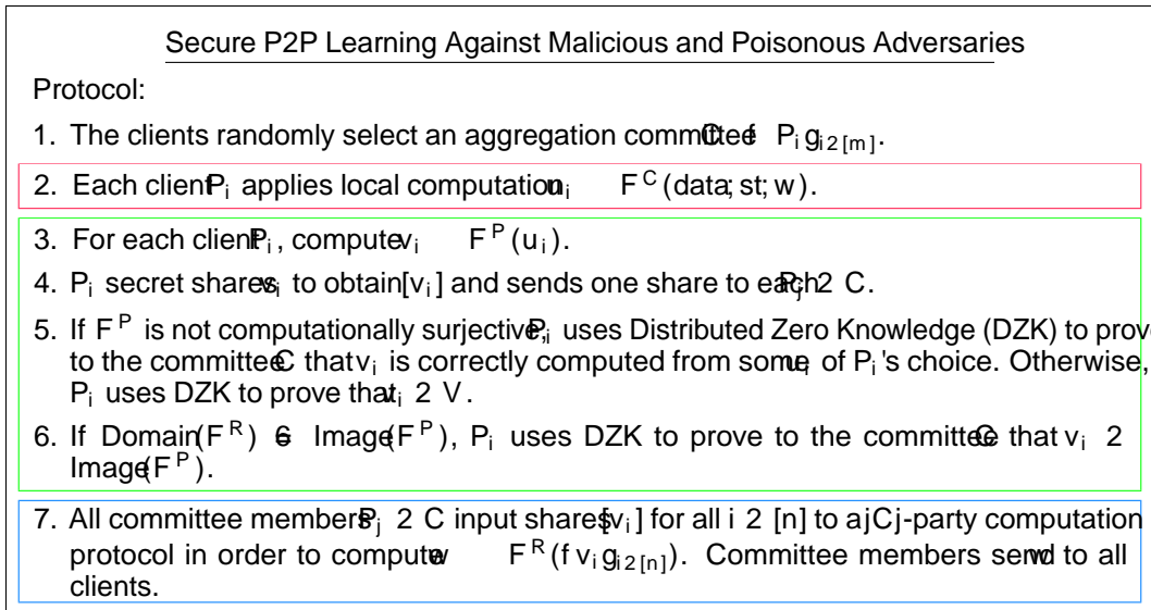
Figure 3: Main protocol outline for the malicious setting.
