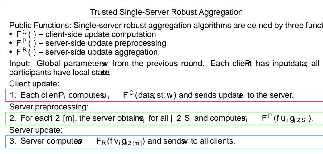
Figure 2: Template for single-server robust aggregation.
