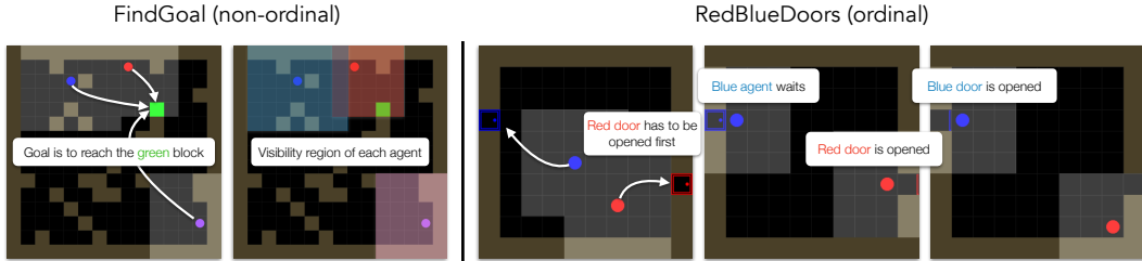
Figure 2: MarlGrid Environment: We introduce two new grid environments: FindGoal (left) and RedBlueDoors (right). These environments are adapted from the GridWorld environment [5, 33]. Environment states are randomized at every episode and are partially observable to the agents. In FindGoal, the task is to reach the green goal location. Each agent receives a reward of 1 when they reach the goal, and an additional reward of 1 when all 3 agents reach the goal within the time frame. In RedBlueDoors, the task is ordinal, where the ordering of actions matter. A reward of 1 is given to both agents if and only if the red door is opened first and then the blue door.
