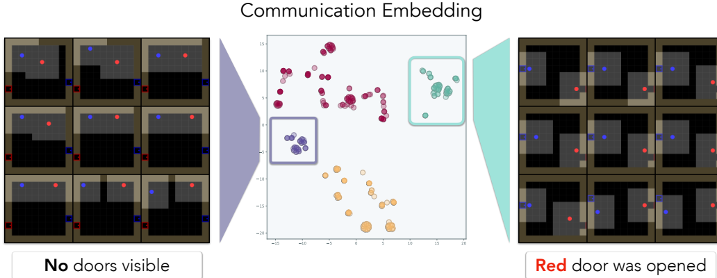
Figure 5: Communication clusters: 4096 communication messages are embedded into low-dimensional representation using t-SNE [44] and is clustered using DBSCAN [11]. We visualize the images corresponding to the communication messages. We observed that the message clusters correspond to various meaningful phases throughout the task. The communication symbol of the purple cluster corresponds to when no doors are visible by either agent, and the light green cluster corresponds to when the red door is opened.
