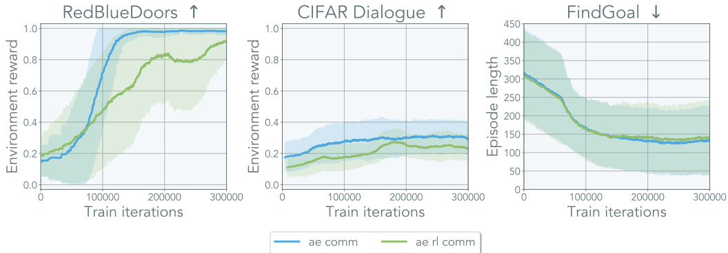
Figure 4: Representation learning with reinforcement learning: Comparison between a speaker module trained with only an autoencoding task ( ae-comm ) and another one trained with both autoencoding task and reinforcement learning ( ae-rl-comm ). We observed that further training a policy on top of the autoencoder representation degrades performance across all environments (except for in FindGoal , where performance of ae-rl-comm and ae-comm stayed about the same).
