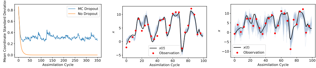
(a) Mean ensemble spread over assimilation cycles (b) Ensemble trajectories with observation noise \sigma = 1.0 (c) Ensemble trajectories with observation noise \sigma = 2.5
