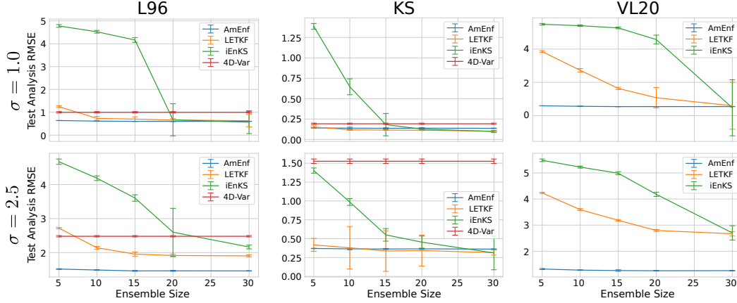
Figure 7: Results from numerical comparisons across multiple ensemble sizes and observation noises.
