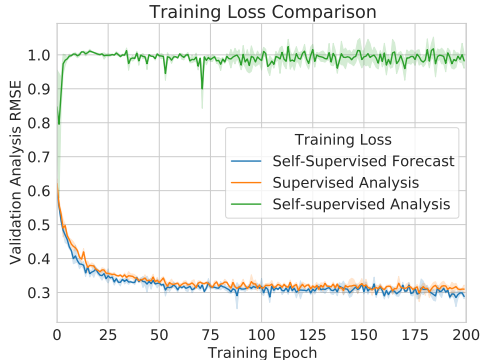
Figure 6: Analysis RMSE evaluated on the validation set across models trained using different losses for \sigma = 1 .
