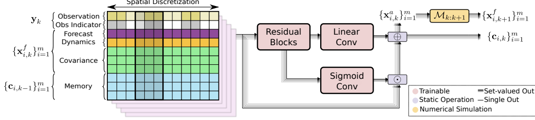
Figure 3: The AmEnF replaces the analysis step of a conventional ensemble filter with a neural network trained using historical data. The model uses an augmented state which includes both standard inputs as well as recurrent memory.
