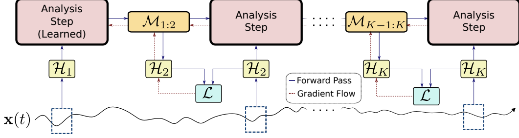
Figure 4: The self-supervised training process is unrolled across multiple filtering steps. Loss is evaluated between “pseudo-observations” and noisy observations obtained from the system.
