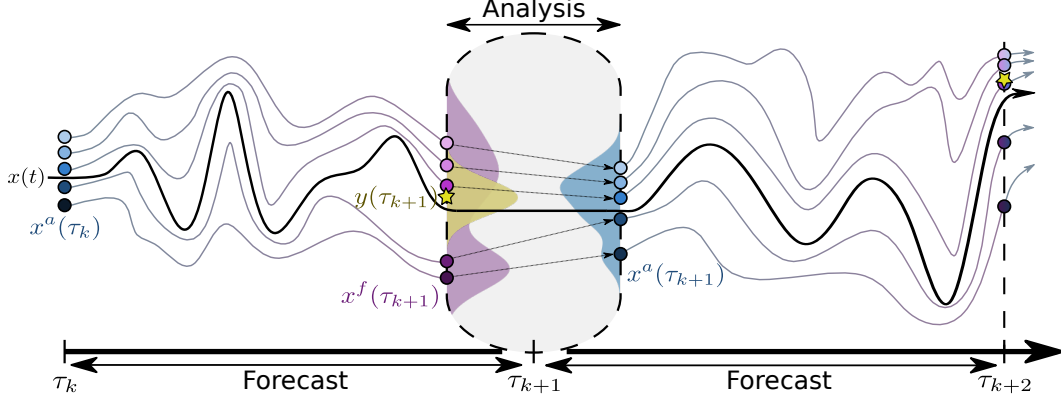
Figure 2: Ensemble filters model the time-evolution of uncertainty under nonlinear dynamics by maintaining a set of samples from the state distribution and simulating their trajectories forward in time. Observations are then used to refine these forecast estimates in what is called the analysis step.
