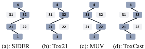
Figure 5: (a)-(d) show the assembled traces (blue links) among located regions (darker blocks) from four meta-testing tasks sampled from SIDER, Tox21, MUV, ToxCast, respectively.
