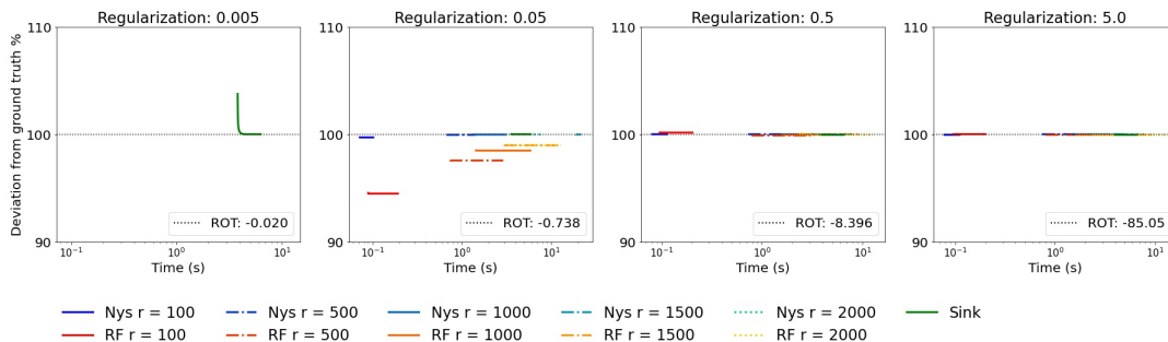
Figure 5: In this experiment, we take randomly 10000 samples from the two distributions of the higgs dataset and we plot the deviation from ground truth for different regularizations. We compare the results obtained for our proposed method ( RF ) with the one proposed in [3] ( Nys ) and with the Sinkhorn algorithm ( Sin ) proposed in [16]. The cost function considered here is the square Euclidean metric and the feature map used is that presented in Lemma 1. The number of random features (or rank) chosen varies from 100 to 2000. We repeat for each problem 10 times the experiment. Note that curves in the plot start at different points corresponding to the time required for initialization. Right, middle right : when the regularization is sufficiently large both Nys and RF methods obtain very high accuracy with order of magnitude faster than Sin . Middle left : both methods manage to obtain high accuracy of the ROT with order of magnitude faster than Sin . Note that Nys performs better in this setting than our proposed method. Left : both methods fail to obtain a good approximation of the ROT.
