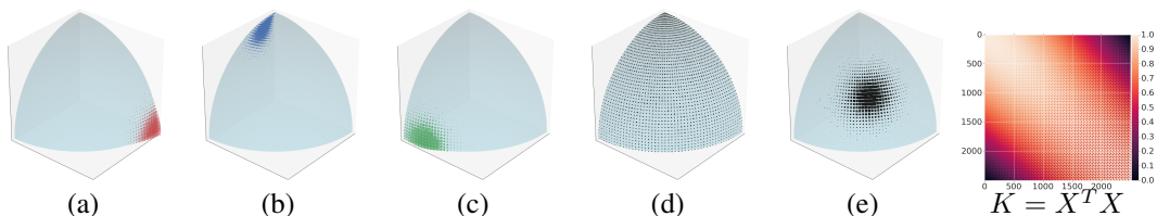
Figure 6: Using a discretization of the positive sphere with 50^2 = 2,500 points we generate three simple histograms (a,b,c) located in the three corners of the simplex. (d) Wasserstein barycenter with a cost c(x, y) = -\log(x^T y) using the method by [9]. (e) Soft-max with temperature 1000 of that barycenter (strongly increasing the relative influence of peaks) reveals that mass is concentrated in areas that would make sense from the more usual c(x, y) = \arccos x^T y distance on the sphere. The kernel corresponding to that cost, here the simple outer product of a matrix X of dimension 3 \times 2500 .
