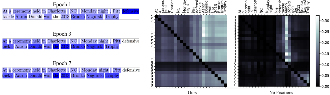
Figure 3: Sentence compression attention maps for both sub-networks (TSM predictions and upstream task attention) in our joint architecture. We show the TSM fixation predictions (left in blue) over epochs (last epoch is our converged models). We show the two-dimensional neural attention maps (right), showing our model and the no fixation model from our ablation study. The two-dimensional maps show the input sequence (horizontal axis) and the predicted sequence (vertical axis). We show the temporal TSM predictions over epochs, in order to depict how the fixation predictions change while training. The fixation predictions (for each epoch, left) are computed over words in the input sequences and then are integrated into the neural attention mechanism which in turn is used to make a prediction (vertical axis, right).
