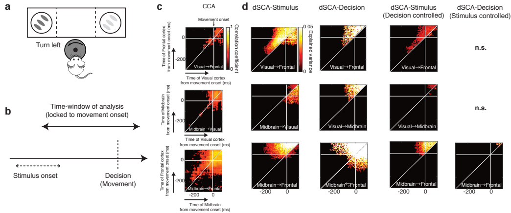
Figure 3: DSCA reveals strong double-dissociation of information sharing between two task parameters that are not apparent by CCA. a Schematic of mice turning a wheel to indicate which of two visual gratings had higher contrast. b Schematic of task sequence. We focus on the time-window of -300 – 100 ms after decision (movement onset). c Results obtained from CCA. Directional arrows indicate significant time lag, whereas bidirectional arrows indicate no significant time lag. d Results obtained from dSCA for sensory inputs (1st column), movement direction (2nd column), sensory inputs that controlled movement direction (3rd column), and movement direction that controlled sensory inputs (4th column). n.s. corresponds to no significant cluster.
