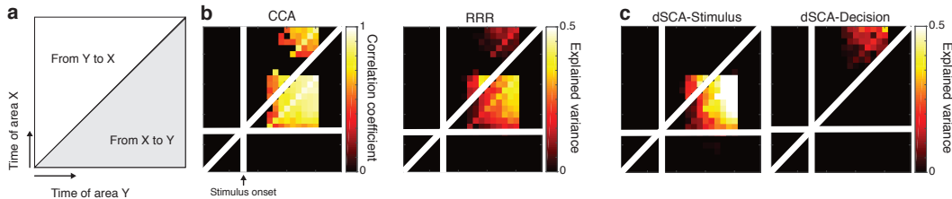
Figure 2: Simulation demonstrates that dSCA decomposes information sharing between different brain regions into different task-relevant parameters. a Schematic of joint peri-event analysis. b Results obtained from CCA (left) and RRR (right) show similar results. c Results obtained from dSCA for stimulus (left) and decision (right).
