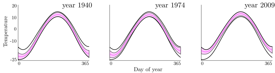
Figure 4: Snapshots from the kernel regression giving yearly temperature curves 1940-2009. We observe an apparent temperature increase which is confirmed by the permutation test.
