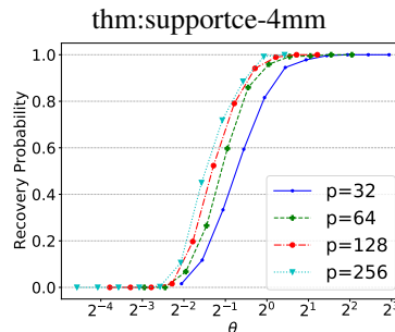
Figure 1: Success probability vs \log \theta .
