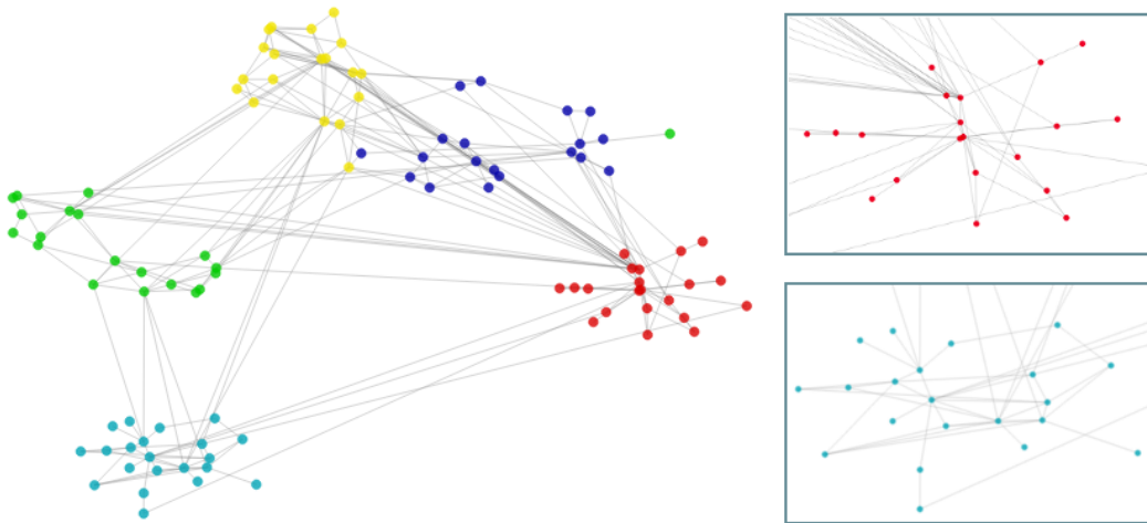
Figure 1: Trained PRODIGE model for a small subset of MNIST dataset, the full graph (left) and a zoom-in of two clusters (right). Vertex positions were computed using tSNE[30] over d_G(\cdot, \cdot) distances; colors represent class labels. View interactively: https://tinyurl.com/prodige-graph
