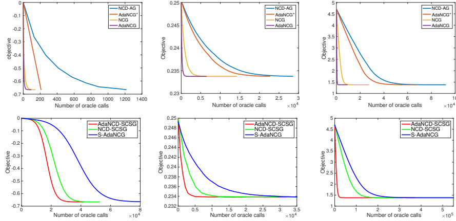
Figure 1: Comparison of different deterministic algorithms (upper) and stochastic algorithms (lower) for solving cubic regularization, regularized nonlinear least square, and neural network (from left to right).
