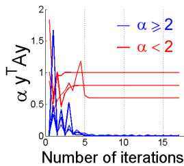
Figure 2: Convergence rate vs. a specific choice of \alpha , averaged over 200 BSD images: \alpha < 2 is marked red, and \alpha \geq 2 is marked blue.
