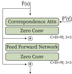
Figure 9: The architecture of the correspondence-aware attention block.
