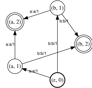
Figure 4: Illustration of the WFA \mathcal{N} for \Delta = \{a, b\} , p = 2 and l = 2 .
