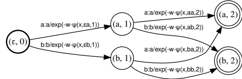
Figure 5: Illustration of the WFA \mathcal{A} for \Delta = \{a, b\} , p = 2 and l = 2 .
