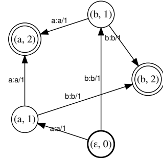
Figure 2: Illustration of the WFA \mathcal{N} for \Delta = \{a, b\} , p = 2 and l = 2 .
