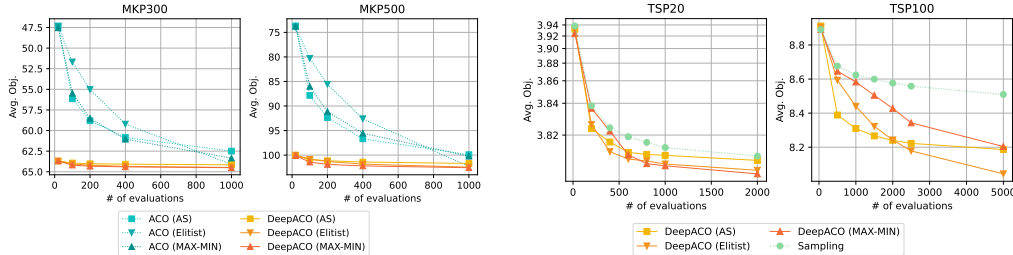
Figure 7: Evolution curves of DeepACO and ACO on MKP300 and MKP500 using the pheromone model PH_{items} .
