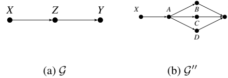
Figure 5: Two causal path graphs generated from (a) the causal graph in Fig. 1a, and (b) the causal graph in Fig. 1b. Both preserve all and only causal paths from \{X\} to \{Y\} in the original graphs.
