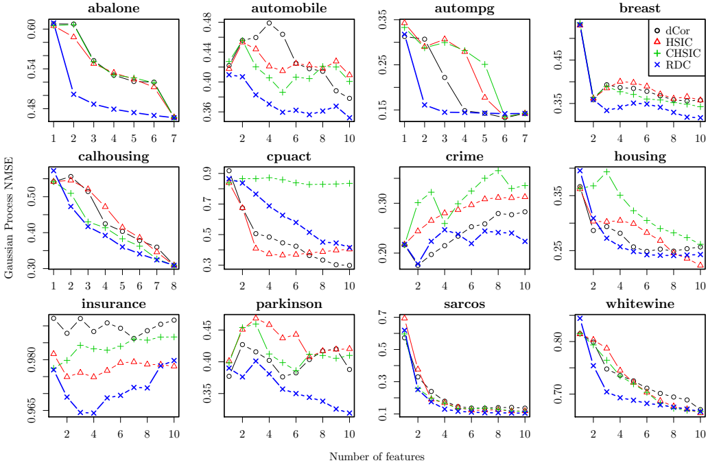
Figure 2: Feature selection experiments on real-world datasets.
