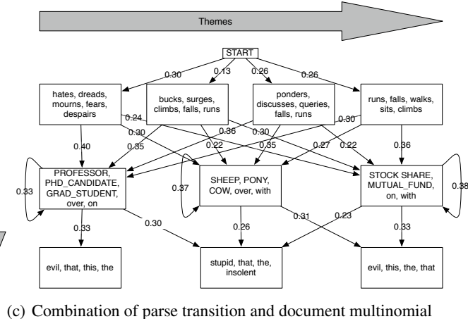
Figure 2: Three models were fit to the synthetic data described in Section 4. Each box illustrates the top five words of a topic; boxes that represent homogenous parts of speech have rounded edges and are shaded. Edges between topics are labeled with estimates of their transition weight \pi . While the infinite tree model (a) is able to reconstruct the parts of speech used to generate the data, it lumps all topics into the same categories. Although the HDP (b) can discover themes of recurring words, it cannot determine the interactions between topics or separate out ubiquitous words that occur in all documents. The STM (c) is able to recover the structure.
